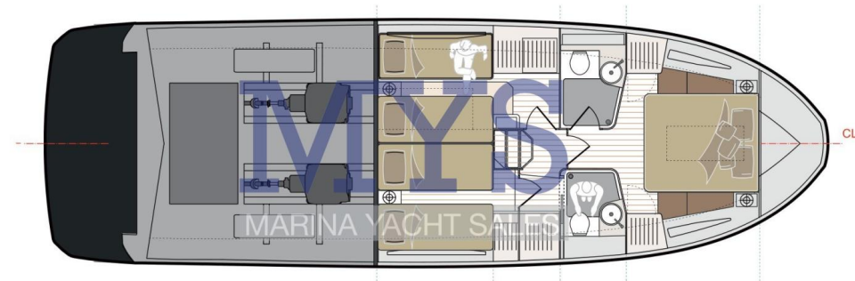
LOWER DECK Three-cabin layout
