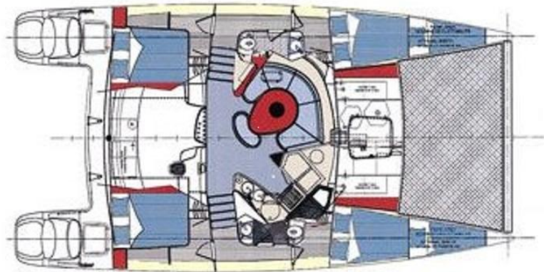
BELIZE 43' Version 4 cabines + 2 salles de bains (4 cabins + 2 bathrooms)
