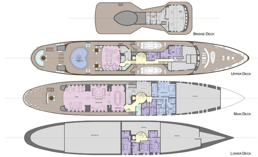
PRIVATE YACHT ENHANCED ACCOMODATION LAYOUT
