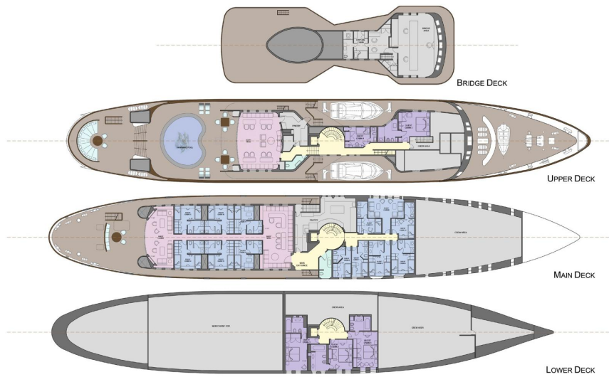
SUPPORT VESSEL LAYOUT
