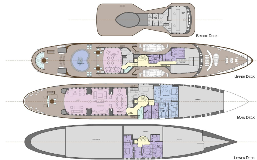
PRIVATE YACHT ENHANCED ACCOMODATION LAYOUT
